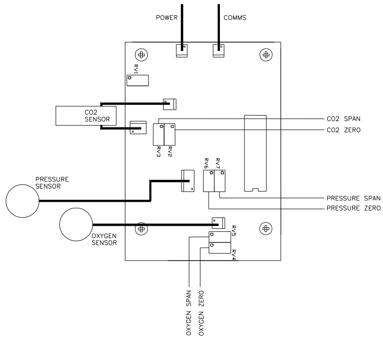
Figure 10: REM1 Calibration pot positions
