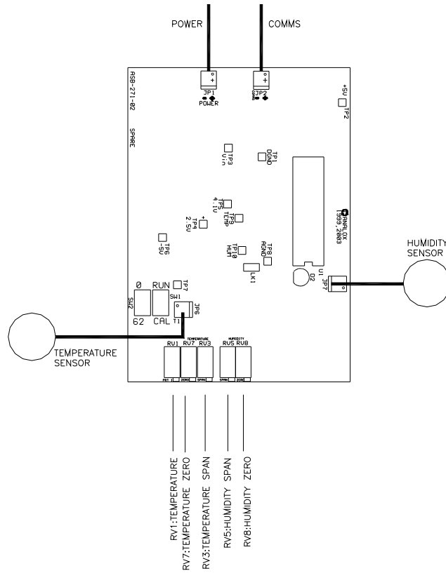
Figure 11: REM2 Calibration pot positions
