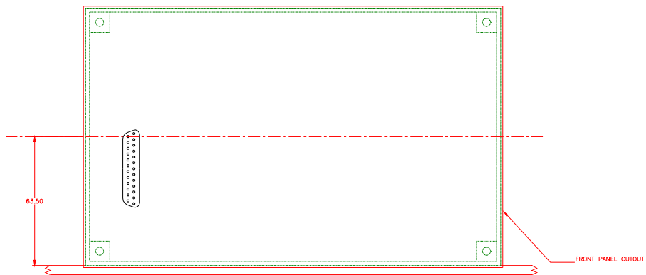
Figure 3: MAIN PANEL REAR SHELF – VIEW FROM REAR
