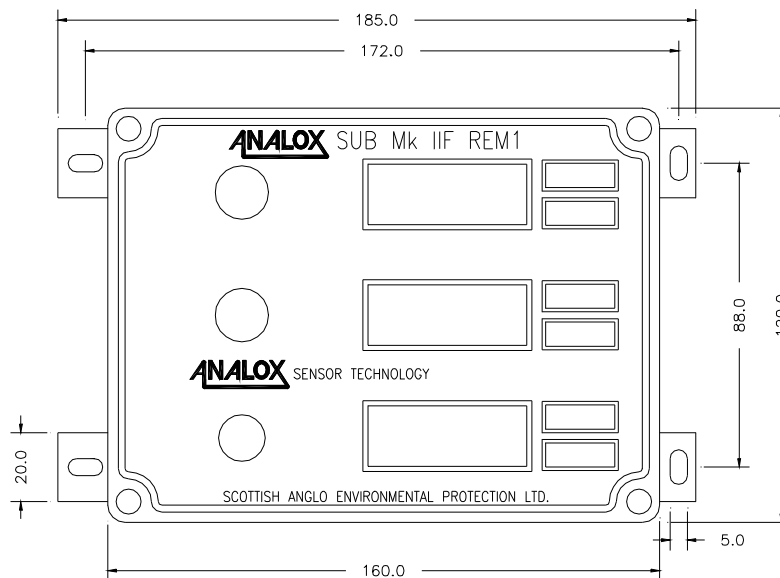
Figure 4: REM MOUNTING DIMENSIONS
