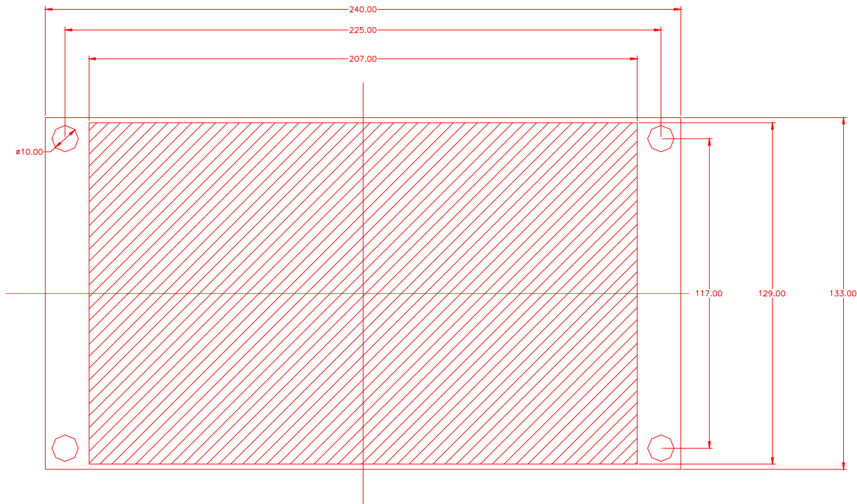
Figure 1: Main Panel - Panel Cutout
