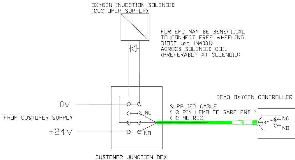
Figure 6: INJECTION CONNECTIONS
