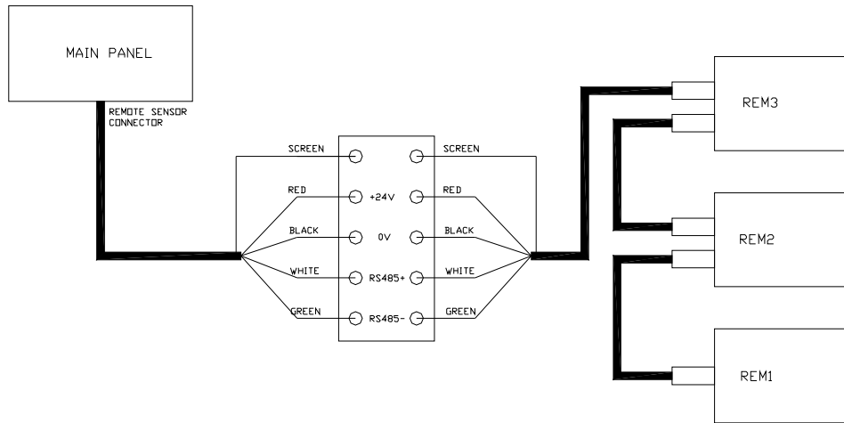
Figure 5: SYSTEM WIRING
