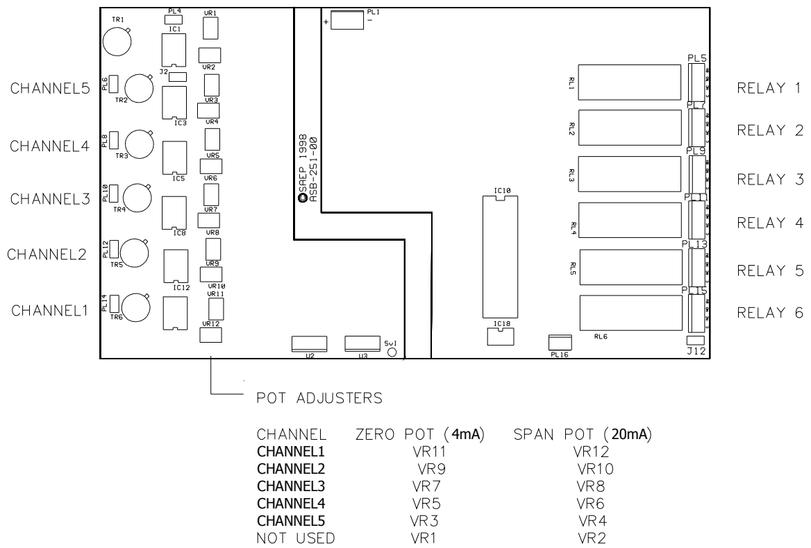
Figure 12: Interface Board - Calibration Pot Positions
