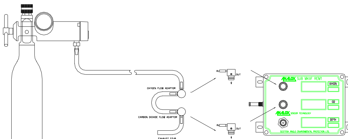
Figure 9: Calibration Arrangement
